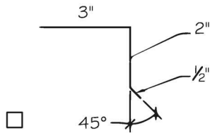
Door Counter Flashing/ Combination Drip Edge Flashing Galvanized 26 ga. (Alternate to Counter Flashing)
