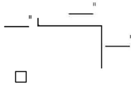
Custom Counter Flashing Galvanized 26 ga. Dimensions Specified by GC (Please dimension above)
