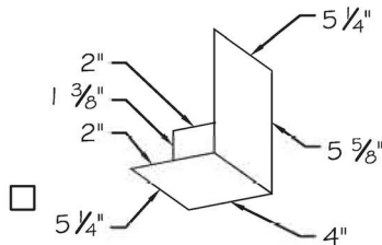
Standard T-Bar End Dams Galvanized 26 ga.
