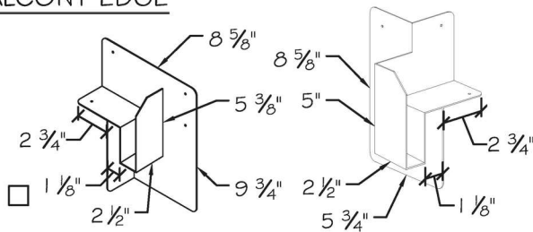
Elevation T-Bar Termination Pockets (TTP)
