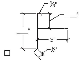
Custom T-Bar Heavy Gauge Aluminum Dimensions Specified by GC (Please dimension above)
