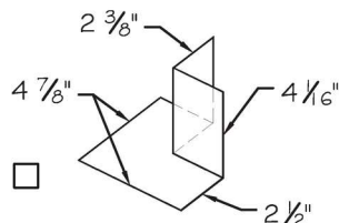
Elevation Combo Pockets Galvanized 26 ga.
