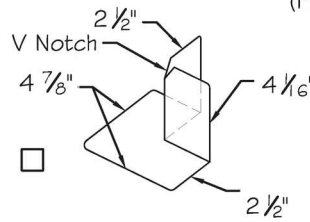
Elevation Poly-Pro Combo Pockets No Sharp corners. Non-corrosive flexible polypropylene
