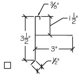
Standard T-Bar Heavy Gauge Aluminum
